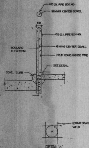
DETAIL OF BOLLARD
